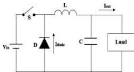
Fig.1.Buckconverter
