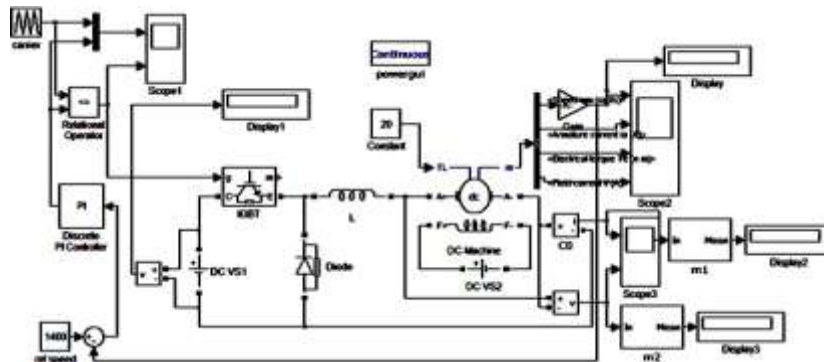
Fig.6. Simulation model of separately excited DC Motor.
