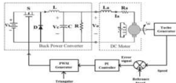
Fig.3. Circuit Diagram
